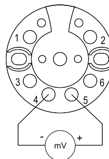
mV SENSOR
